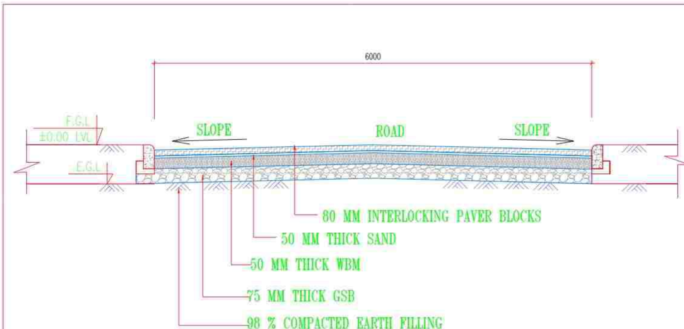
TYPICAL CROSS SECTION FOR PAVERS BLOCK ROAD
