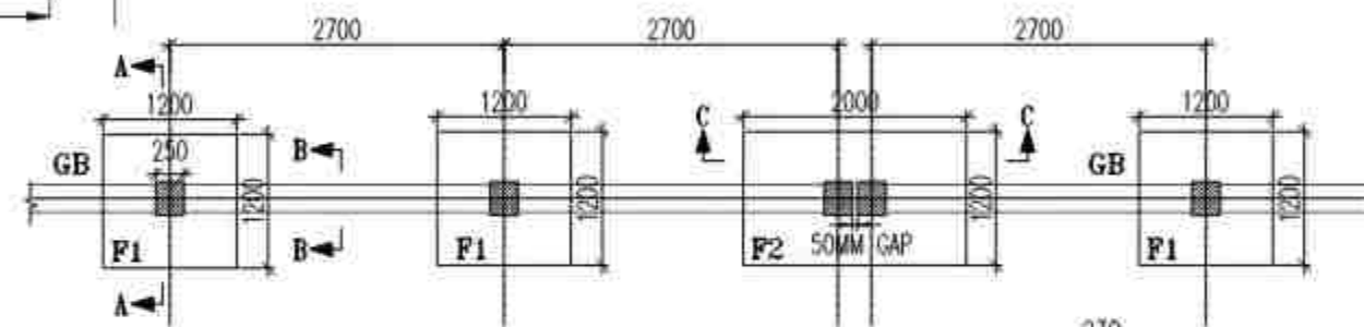
BOUNDARY WALL PLAN * EXPANSION JOINT SHOULD BE PROVIDED AT EVERY 27 METER LENGTH
