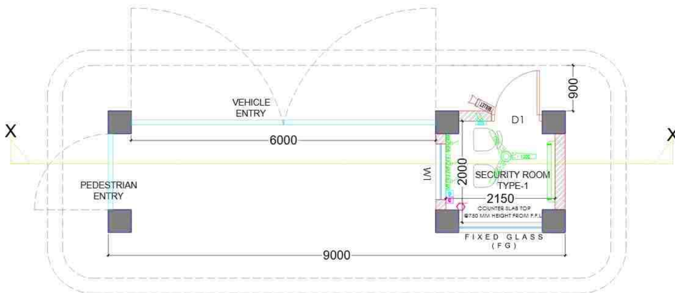
MAIN GATE PLAN-1
