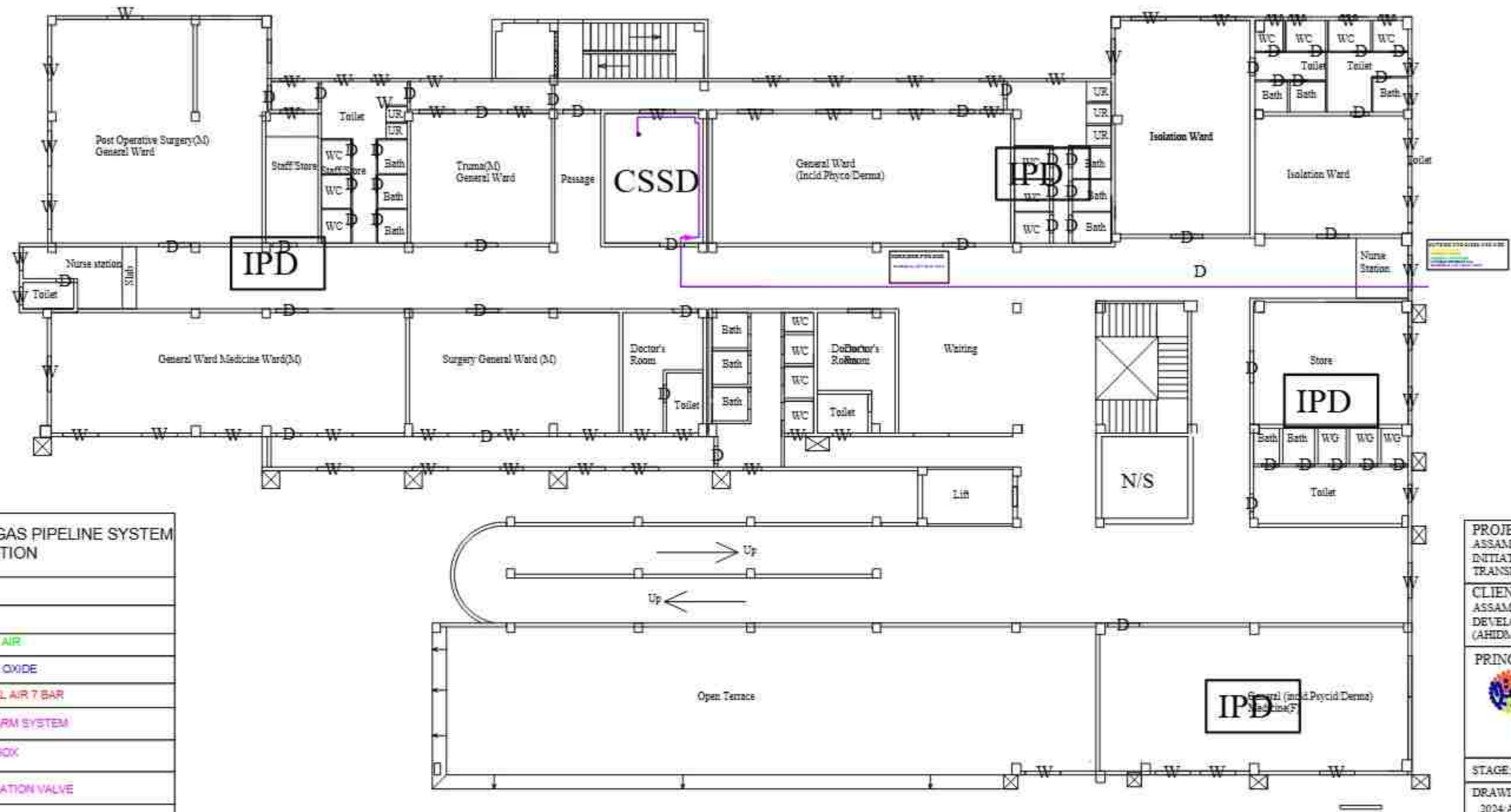
2nd Floor
